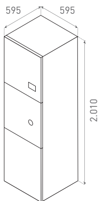
INTEGRRA 150/40
